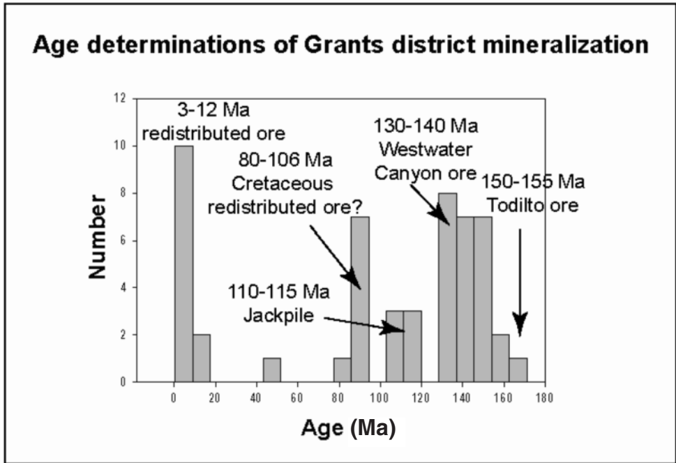
Figure 6. Age determinations of Grants district mineralization. Includes Pb/U, K/Ar, Rb/Sr, and fission track dates from Miller and Kulp (1963), Nash and Kerr (1966), Nash (1968), Berglof (1970, 1989), Brookins et al. (1977), Brookins (1980), Ludwig et al. (1982), Hooper (1983) and is summarized by Wilks and Chapin (1997).
