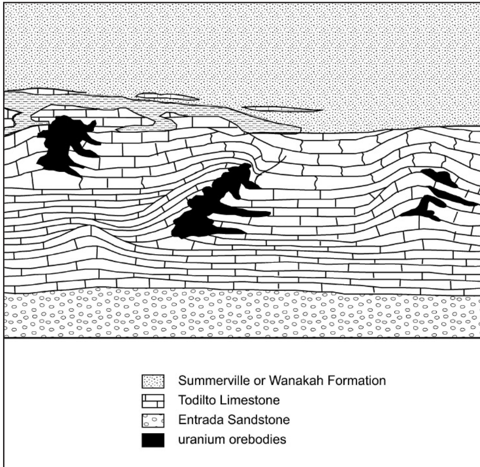
Figure 4. Control of Todilto uranium deposits by intraformational folds and fractures (modified from Finch and McLemore, 1989).
